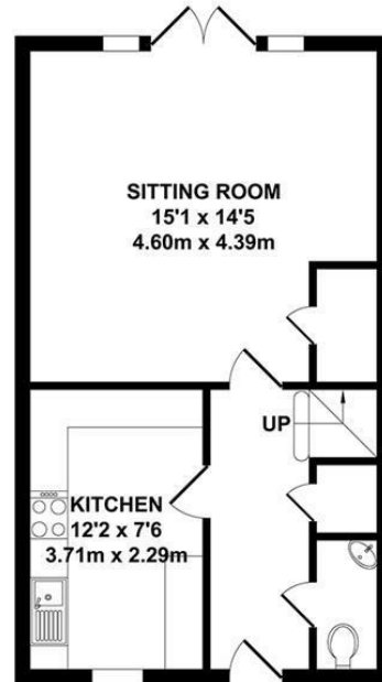
GROUND FLOOR APPROX. FLOOR AREA 406 SQ.FT. (37.72 SQ.M.)
